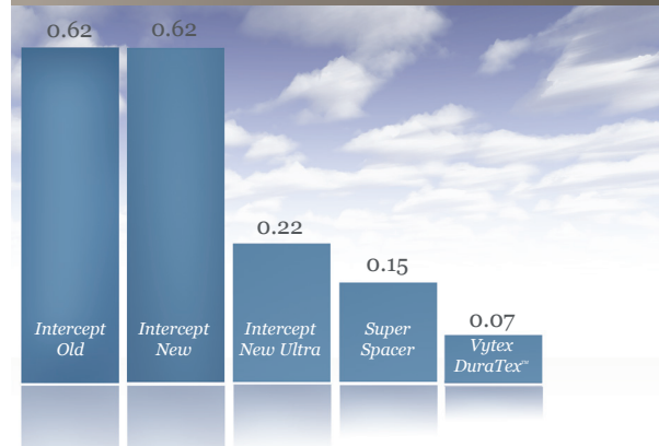
The lower the thermal conductivity, the warmer the glass—and the more comfortable you feel. Vytex DuraTex™ Warm Edge Spacer System offers a 50% improvement in thermal conductivity over Super Spacer and an 80% improvement over Intercept.
