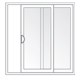
Two-panel widths: 5', 6', 8'
