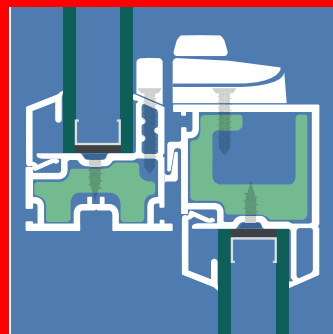
Composite Reinforced Interlocking Sashes
