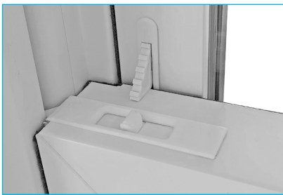
Vent Stop, when deployed, will limit sash travel to allow for ventilation.
